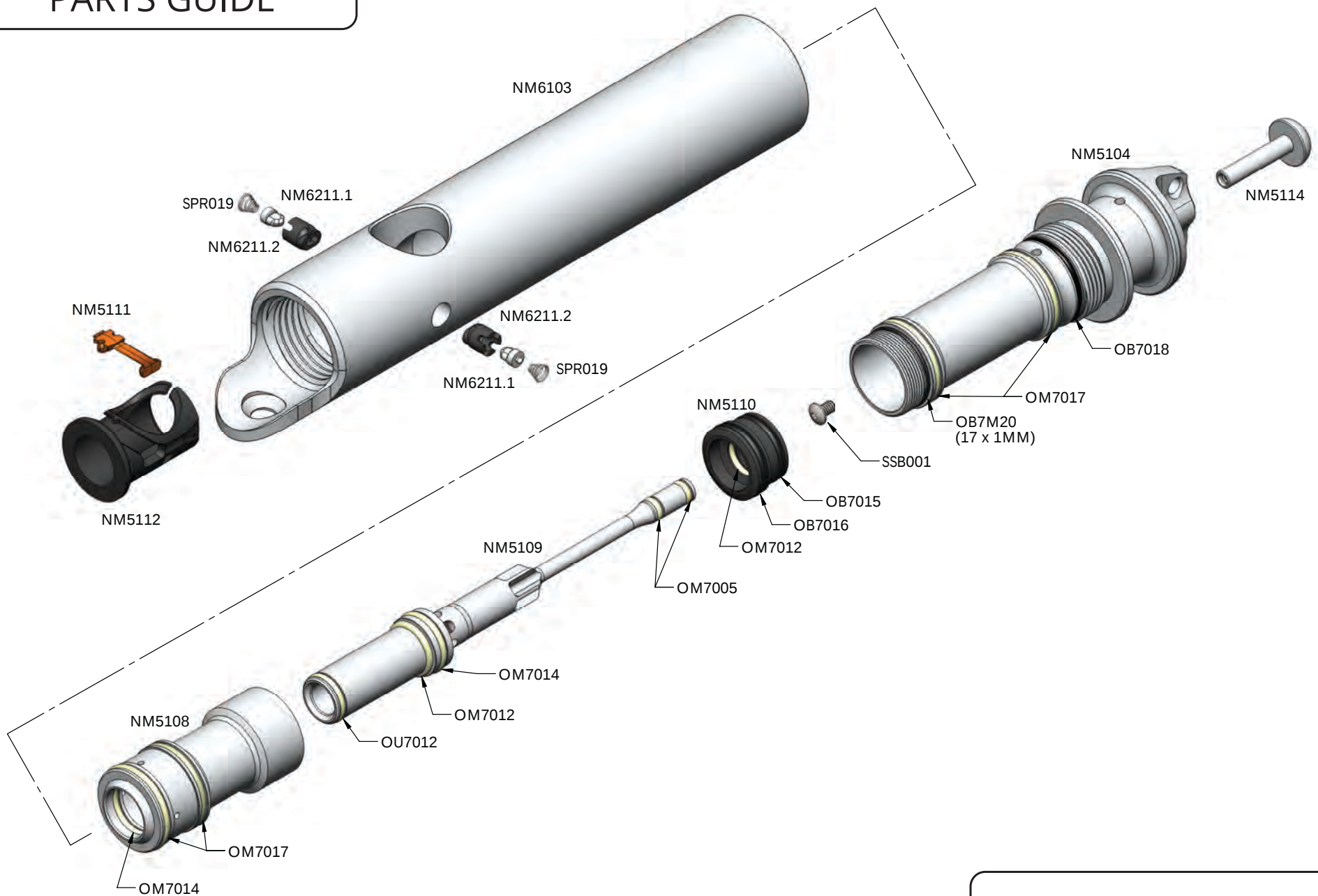
FIGURE 4 50 CAL. INTERNALS
