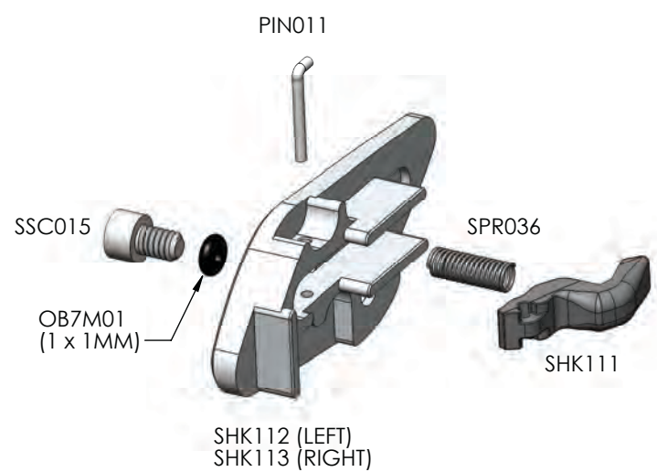
BALL DETENT
