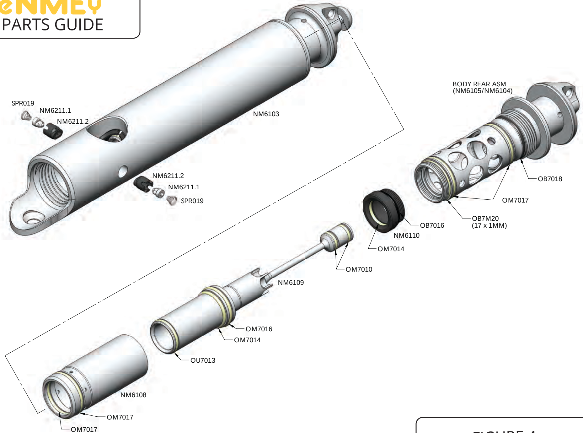
FIGURE 4 68 CAL. INTERNALS
